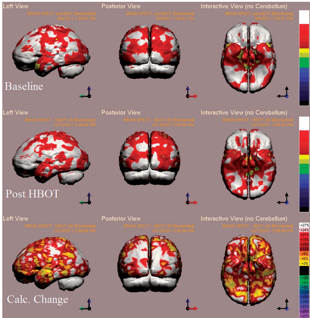
Fig. 8. Case 5 SPECT calculated change after HBO 2 compared to baseline. In the first two rows color represent maximal brain activity relative to brain median activity, where in the bottom row colors represent the change in regional brain function i.e. the change in metabolic activity. A global improvement of brain activity is demonstrated more accentuated in both occipital cortices. White and red areas show the highest changes in CBF. Executive function and attention indices improved from 44 and 38 to 62 and 59, respectively.
